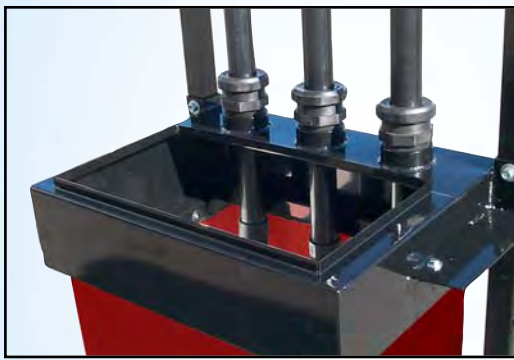
Standard water-splash lip prevents water intrusion beneath the cover
